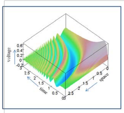
Figure 1. Theoretical voltage responses to an impulsive stimulus. For an explanation of the parameters (here \phi=\pi/2 , a=1 , \varepsilon=1 , and \sigma=1 ).used see Appendix A.
